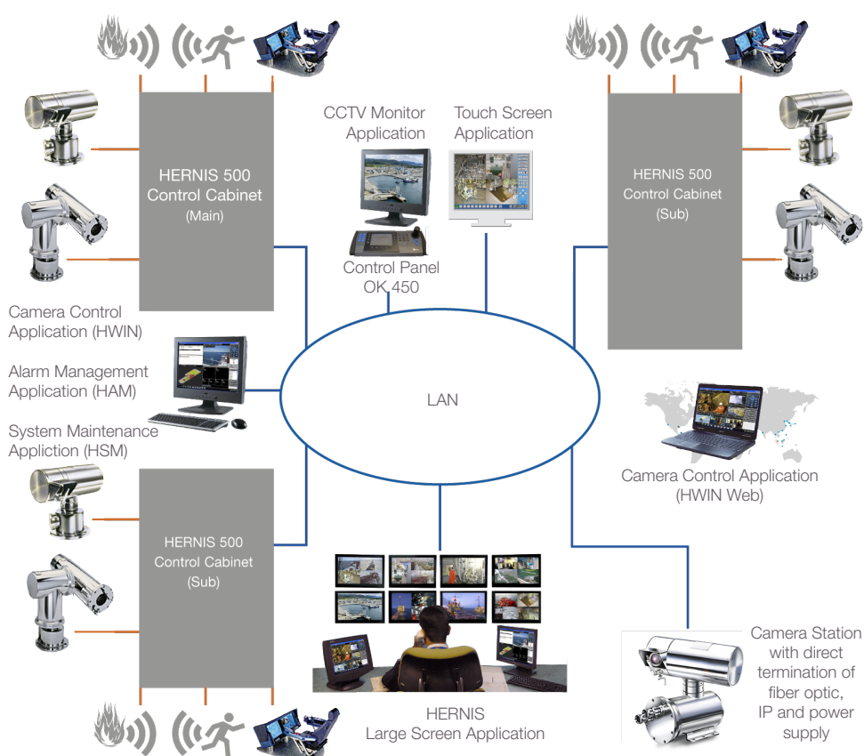
HERNIS 500 architecture
